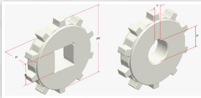
Square Bore Sprockets
