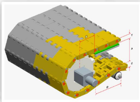
HS-1800A (General Assembly Line)
