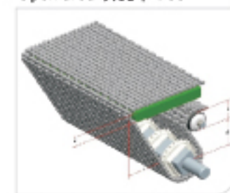
Type 型号: HS-400B Pitch 节距: 10MM Thickness 厚度: 7MM Open area 开孔率: 24%
