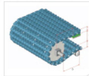
Type 型号: HS-1700B Pitch 节距: 38.1MM Thickness 厚度: 18.9MM Open area 开孔率: 37%
