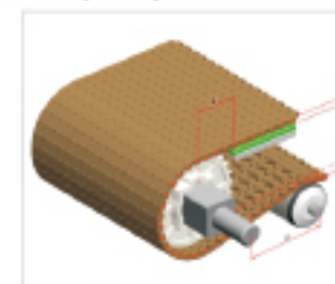
Type 型号: HS-1500A-HD Pitch 节距: 12.7MM Thickness 厚度: 10MM Open area 开孔率: 0%
