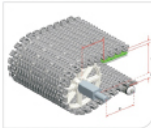
Type 型号: HS-1200B Pitch 节距: 31.75MM Thickness 厚度: 12MM Open area 开孔率: 40%
