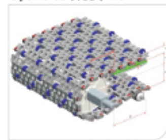
Type 型号: HS-300C Pitch 节距: 45MM Thickness 厚度: 19.5MM Open area 开孔率: 52%
