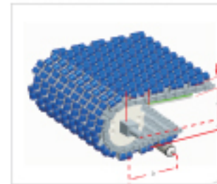
Type 型号: HS-1700C Pitch 节距: 38.1MM Thickness 厚度: 47.6MM Open area 开孔率: 26%
