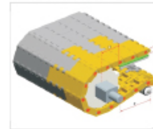
Type 型号: HS-1800A Pitch 节距: 63.5MM Thickness 厚度: 25MM Open area 开孔率: 0%
