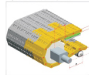
Type 型号: HS-1800B Pitch 节距: 50.8MM Thickness 厚度: 20MM Open area 开孔率: 11%
