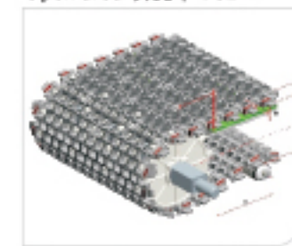
Type 型号: HS-300B-PLUS-EL Pitch 节距: 45MM Thickness 厚度: 18MM Open area 开孔率: 52%
