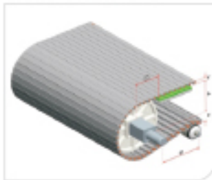
Type 型号: HS-1100A Pitch 节距: 15.2MM Thickness 厚度: 9MM Open area 开孔率: 0%
