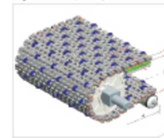
Type 型号: HS-500C Pitch 节距: 25.4MM Thickness 厚度: 13.5MM Open area 开孔率: 36%
