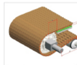
Type 型号: HS-1500A Pitch 节距: 12.7MM Thickness 厚度: 8.5MM Open area 开孔率: 0%
