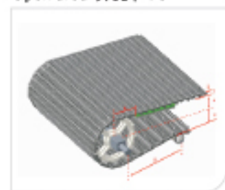
Type 型号: HS-103B-HD-AN Pitch 节距: 50.8MM Thickness 厚度: 19MM Open area 开孔率: 27%
