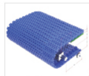
Type 型号: HS-1201B Pitch 节距: 31.75MM Thickness 厚度: 12.5MM Open area 开孔率: 36%
