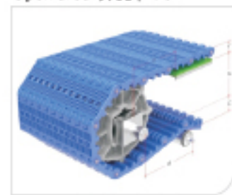
Type 型号: HS-102B Pitch 节距: 50.8MM Thickness 厚度: 16MM Open area 开孔率: 20%
