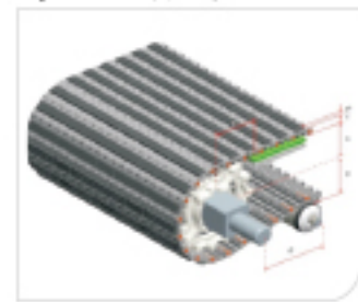
Type 型号: HS-200EL Pitch 节距: 25.4MM Thickness 厚度: 13MM Open area 开孔率: 0%
