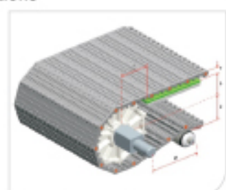
Type 型号: HS-100B Pitch 节距: 50.8MM Thickness 厚度: 16MM Open area 开孔率: 20%
