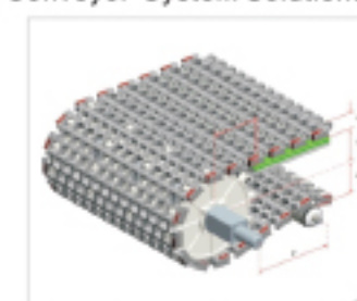
Type 型号: HS-300B Pitch 节距: 45MM Thickness 厚度: 15MM Open area 开孔率: 52%
