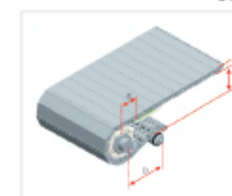
Type 型号: HS-6800A Pitch 节距: 38.1MM Thickness 厚度: 19MM Open area 开孔率: 0%
