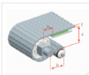
Type 型号: HS-1001B Pitch 节距: 19MM Thickness 厚度: 8.5MM Open area 开孔率: 27%
