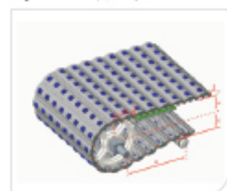
Type 型号: HS-100A-HD-N-C Pitch 节距: 50.8MM Thickness 厚度: 26.5MM Open area 开孔率: 3%
