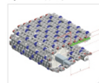
Type 型号: HS-300B-HD-C Pitch 节距: 45MM Thickness 厚度: 19.5MM Open area 开孔率: 38%
