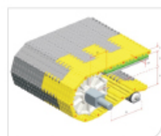
Type 型号: HS-100D Pitch 节距: 50.8MM Thickness 厚度: 17.3MM Open area 开孔率: 0%
