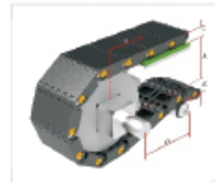
Type 型号: HS-1800A-100 Pitch 节距: 63.5MM Thickness 厚度: 25MM Open area 开孔率: 0%
