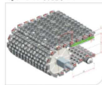
Type 型号: HS-300B-EL Pitch 节距: 45MM Thickness 厚度: 18MM Open area 开孔率: 52%
