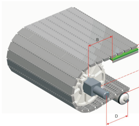
Conveyor Frame Dimensions
